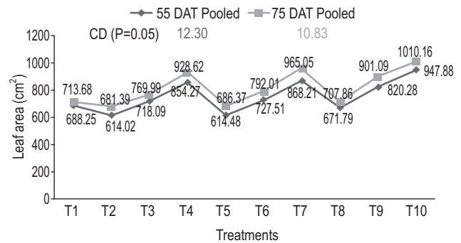
Fig. 4 Effect of P. fluorescens , humic acid and level of fertilizers on leaf area of cabbage at different days after transplanting (DAT)
