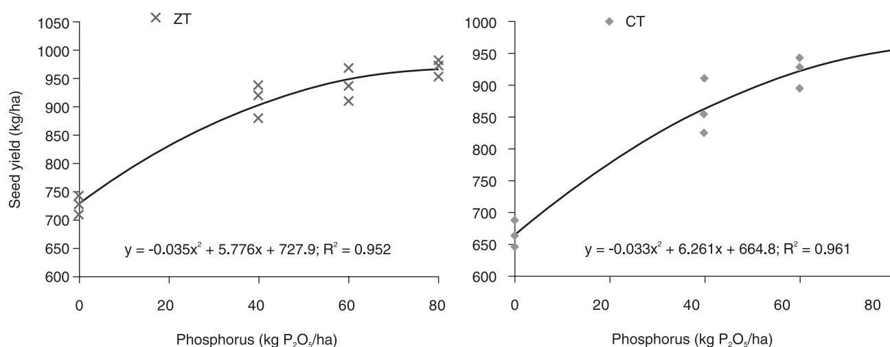
Fig 1 Quadratic regression between seed yield of mungbean and applied phosphorus doses under contrasting tillage practices.
