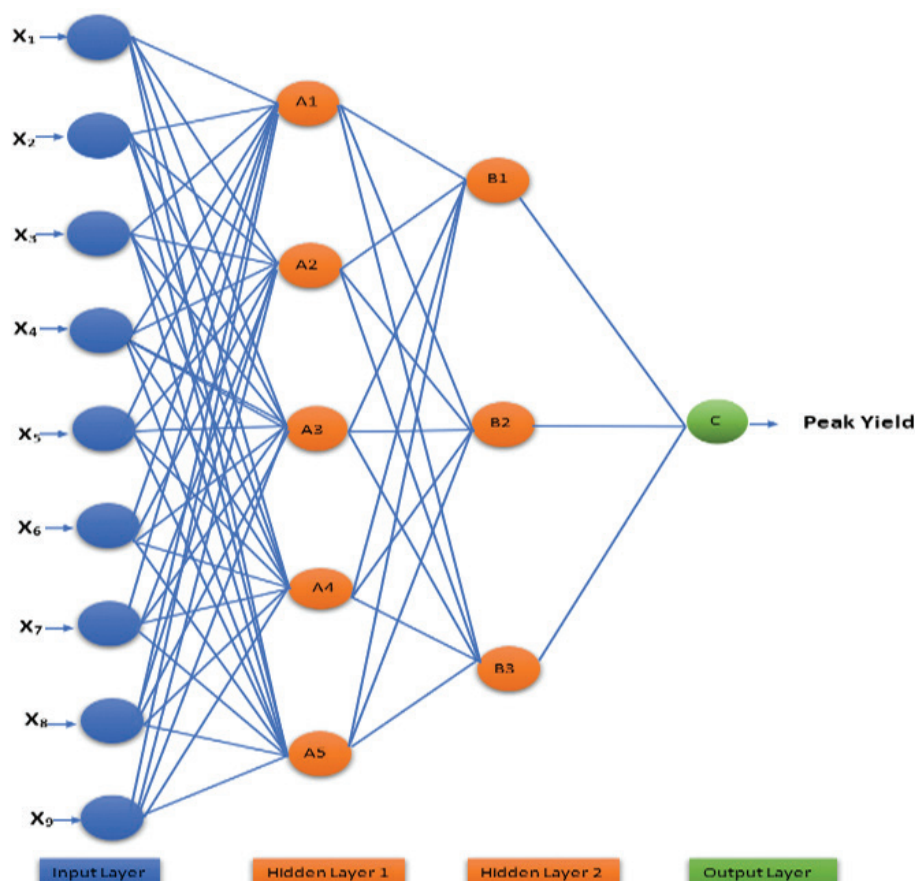
Supplementary Figure 1. Graphical representation of optimal ANN model
