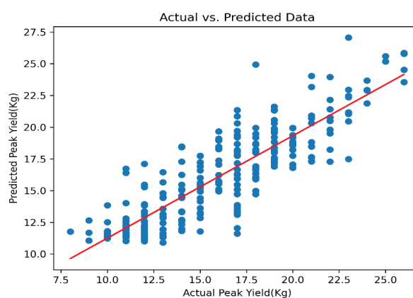
Supplementary Figure 2. Predicted vs actual peak yield using ANN model
