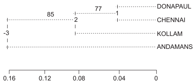
Fig. 3. UPGMA dendrogram showing relationships in P. viridis from various locations using Popgene software.
