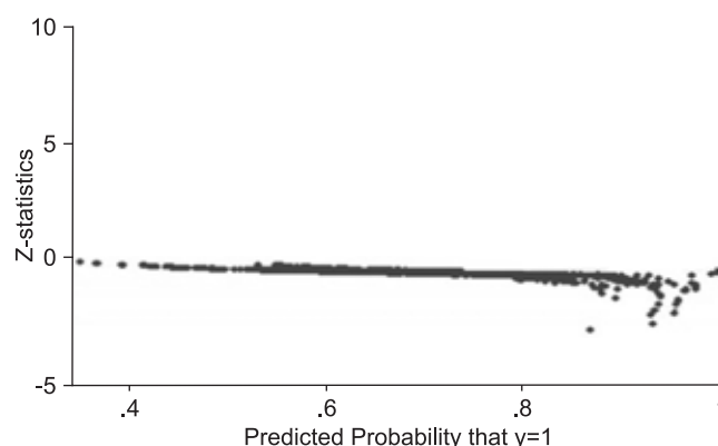
Fig. 1. Z-statistics of interaction effect (literacy of head of household and herd size of milch dairy animals) after logit .
