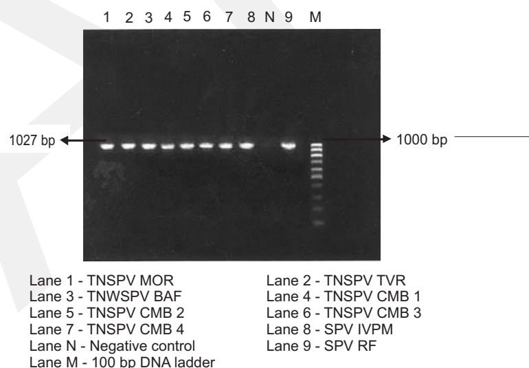
Fig 1. Agarose Gel electrophoresis of full length sheep poxviral P32 gene
