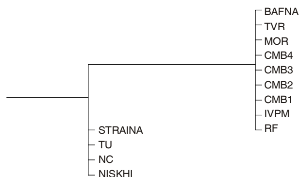
Fig. 2. Phylogenetic analysis of Indian and foreign strains of sheep poxvirus
