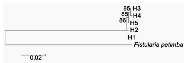
Fig 1. Evolutionary relationship of Hippocampus kuda populations based on 16S rRNA sequence data (Neighbour-Joining method).
