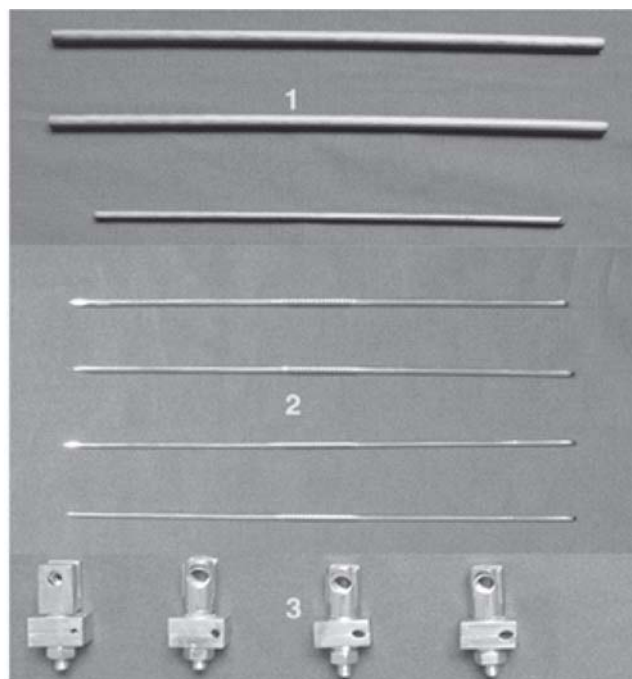
Fig. 1. External skeletal fixator components. 1, Carbon fiber connecting rods (6.3mm and 4mm); 2, centrally threaded trans fixation pins (3mm and 2.5mm); 3, connecting 2-way AO clamps.
