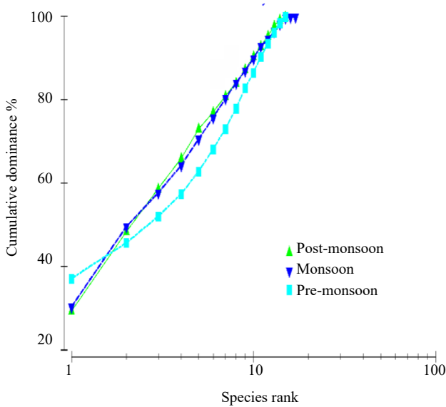
Fig. 2. Dominance plot (Temporal scale)
