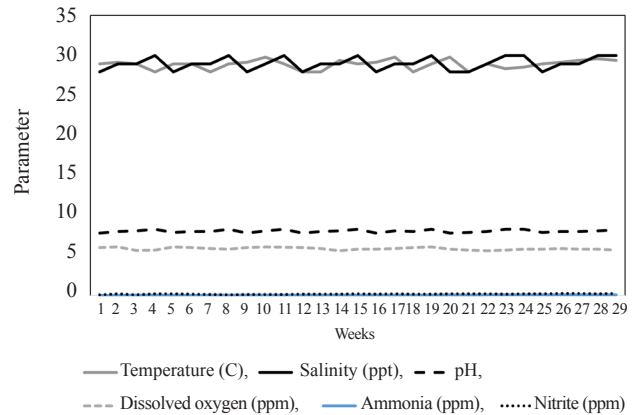
Fig. 2. Water quality parameters recorded during the farming of snubnose pompano in RAS system
