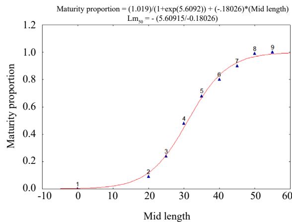
Fig. 4. Length at first maturity ( L_{m50} ) of male S. obtusata
