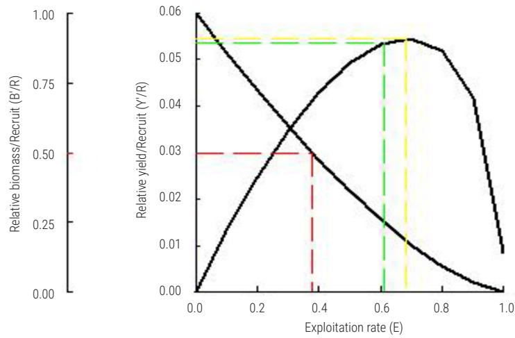
Fig. 8. Stock status of A. hians using Beverton and Holt's relative Y/R model.
