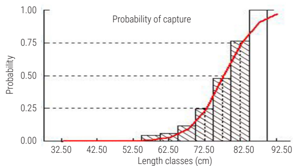
Fig. 6. Length at capture ( L_{50} ) of A. hians from Kerala coast
