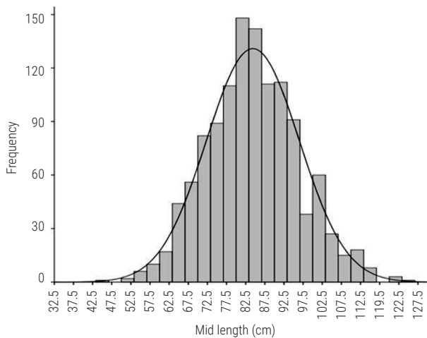
Fig. 2. Length frequency distribution of A. hians collected between 2015 and 2017 along Kerala coast
