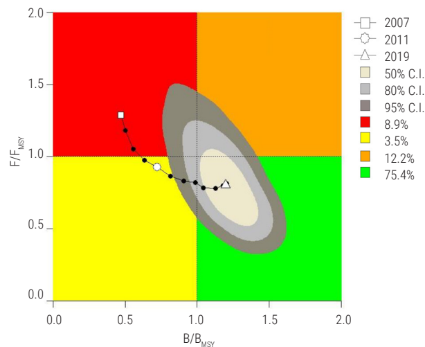
Fig. 4. KOBE plot indicating the stock status of the resource based on BSM analysis
