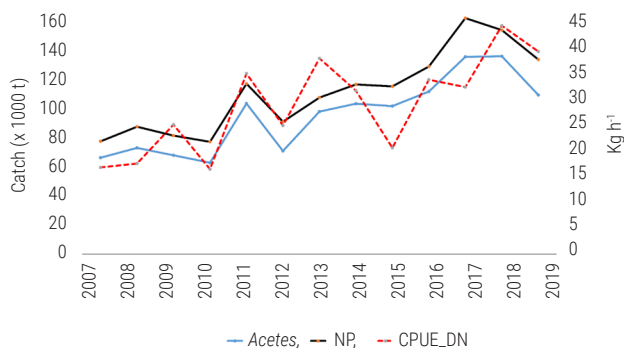
Fig. 1. Time series catch trend of Acetes and non-penaeid shrimps (NP) and abundance indices (CPUE_DN) for Acetes along Gujarat coast
