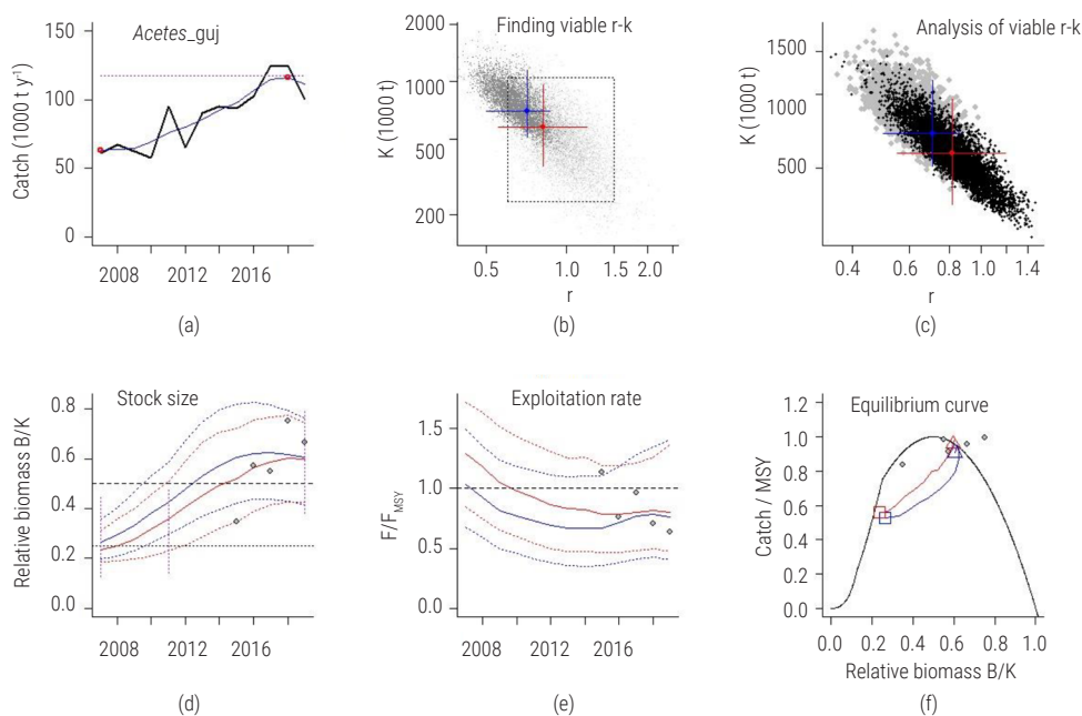
Fig. 3. Output of CMSY and BSM for Acetes landed along the Gujarat coast (2007-19)
