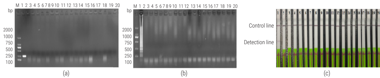
Fig. 2. V. vulnificus LAMP-LFD specific assay. (a) Agarose gel electrophoresis of PCR products; (b) agarose gel electrophoresis of LAMP products; (c) LAMP-LFD. Lane M: DL2000 DNA Marker, lane 1~20: V. vulnificus , V. harveyi , V. alginolyticus , V. parahaemolyticus , V. fluvialis , V. campbellii , V. furnissii , V. cholerae , E. faecalis , K. trevisan , E. hormaechei , B. licheniformis , A. radioresistens , P. mirabilis , E. coli , A. hydrophila , S. aureus , B. cereus , P. aeruginosa , S. agalactiae
