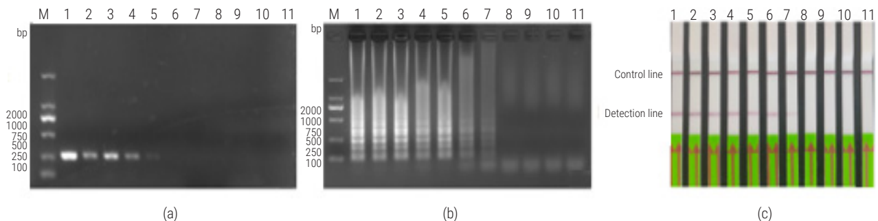
Fig. 3. Comparison of sensitivity for the detection of V. vulnificus between PCR (a) LAMP; (b) LAMP-LFD; (c) Lane M: DL2000 DNA Marker, Lane 1~11: 20.0 \text{ ng } \mu\text{L}^{-1} \sim 2.0 \times 10^{-9} \text{ ng } \mu\text{L}^{-1} for 10-fold dilution.
