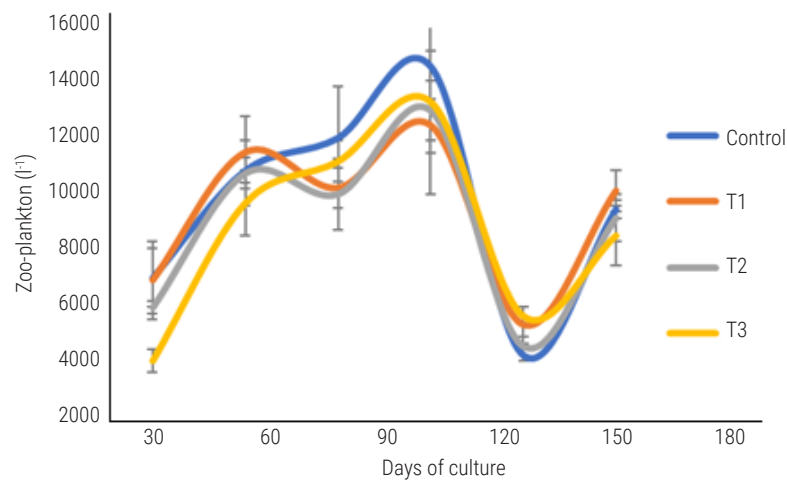
Fig. 5. Zooplankton abundance in the experimental ponds under different treatments during culture period
