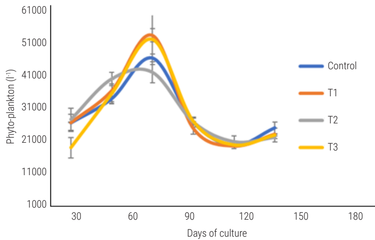
Fig. 4. Phytoplankton abundance in the experimental ponds under different treatments during culture period
