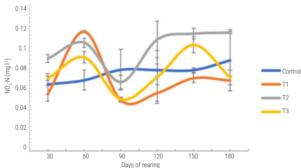
Fig. 2. Level of \text{NO}_2\text{-N} in the experimental ponds under different treatments during culture period
