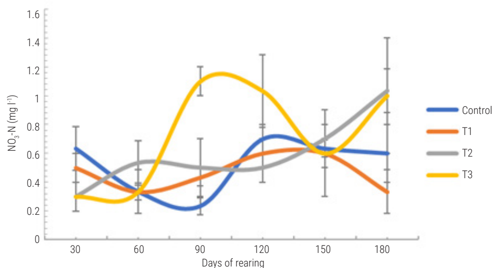
Fig. 3. Level of \text{NO}_3\text{-N} in the experimental ponds under different treatments during culture period
