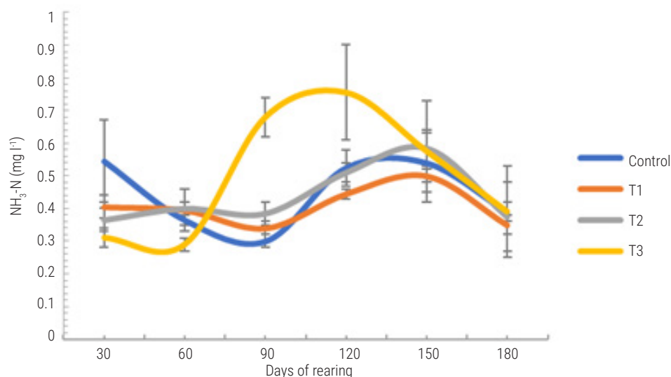
Fig. 1. Level of \text{NH}_3\text{-N} in the experimental ponds under different treatments during culture period
