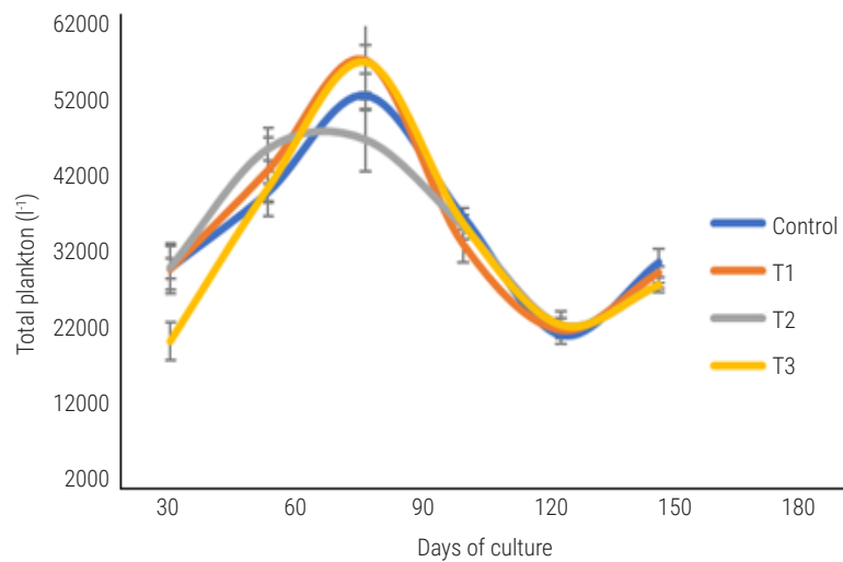
Fig. 6. Total plankton abundance in the experimental ponds under different treatments during the culture period
