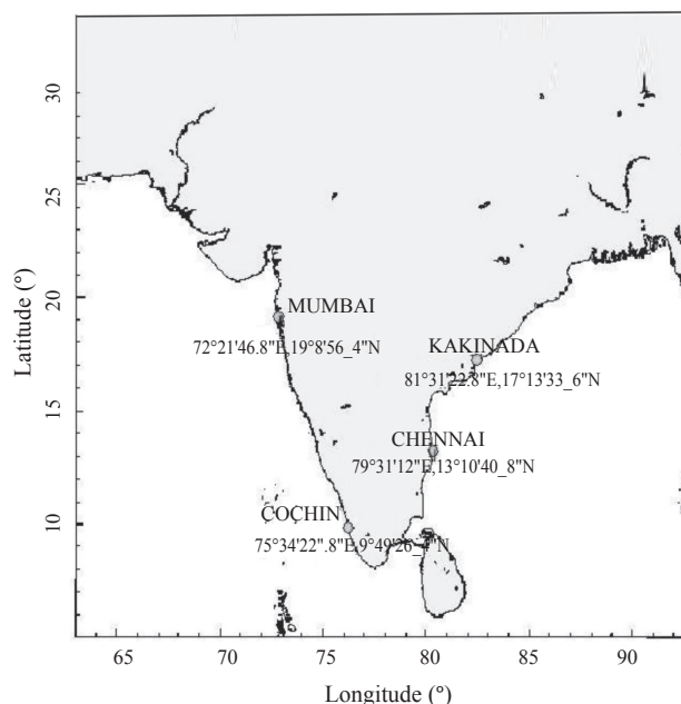
Fig. 1. Locations selected for sampling of N. japonicus
