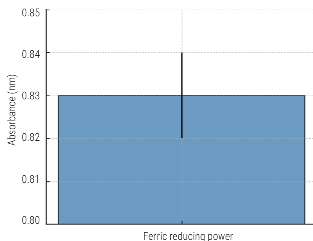
Fig. 2. Ferric reducing antioxidant power of the jellyfish body fluid
