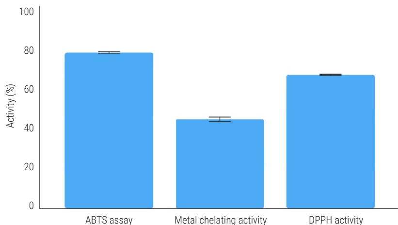
Fig. 1. ABTS radical scavenging activity, metal chelating activity and DPPH activity of the jellyfish body fluid
