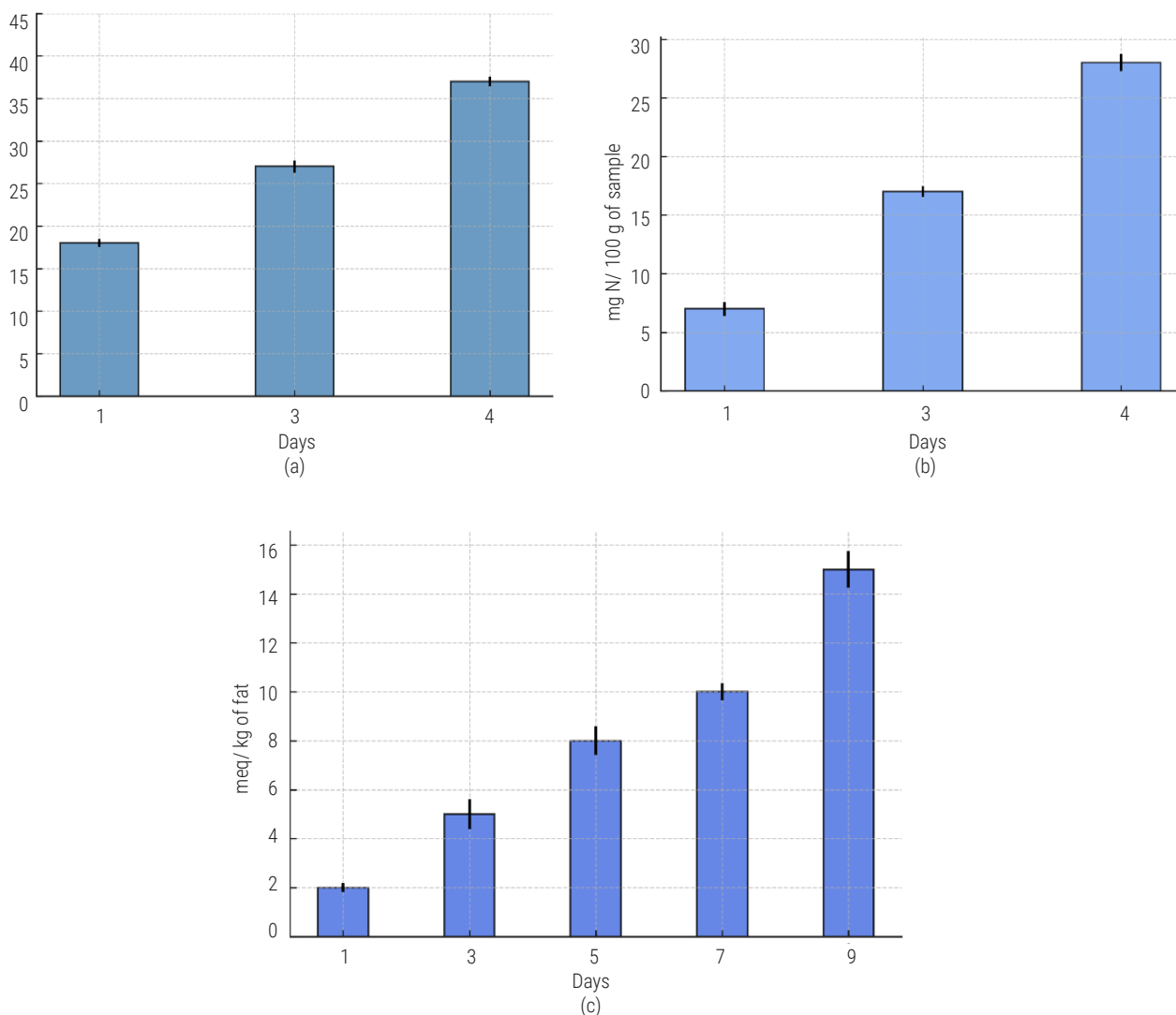
Fig. 3. (a) TVBN ; (b) TMA and (c) Peroxide values of jellyfish during storage
