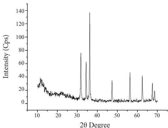
Fig. 1a. XRD pattern of S 70 ZnO NPs
