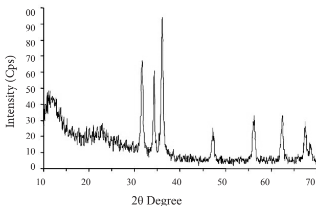
Fig. 1b. XRD pattern of S 83 ZnO NPs
