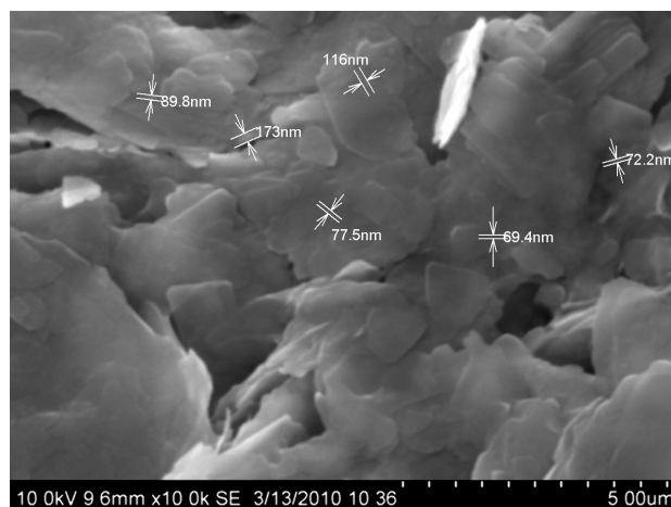
Fig. 2b. SEM image of S 83 ZnO NPs
