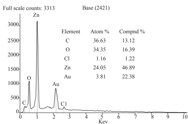
Fig. 3b. EDAX Spectrum of S 83 ZnO NPs
