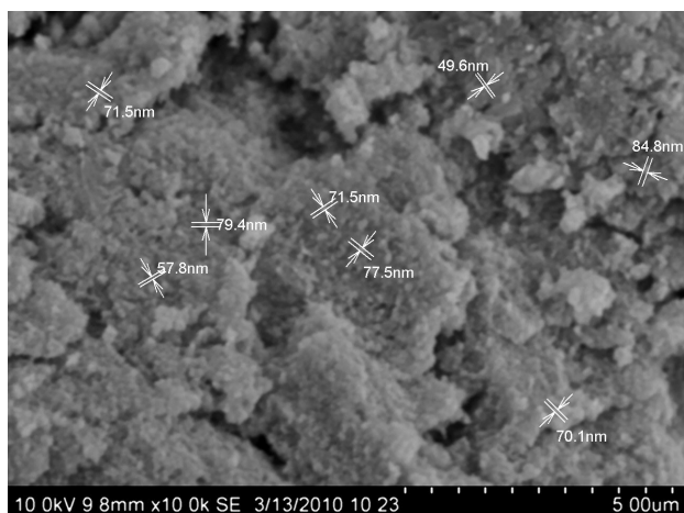
Fig. 2a. SEM image of S 70 ZnO NPs
