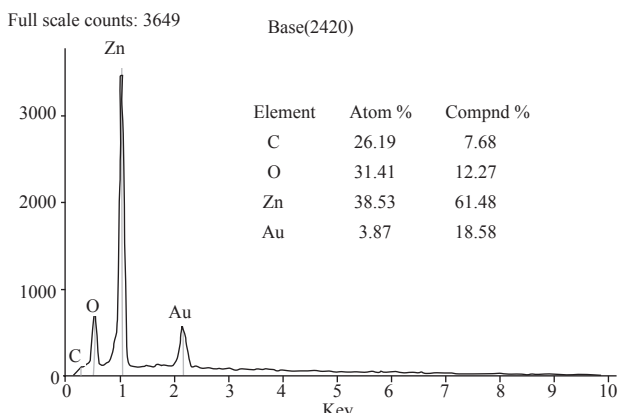
Fig. 3a. EDAX Spectrum of S 70 ZnO NPs
