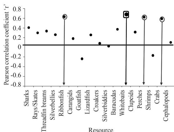
Fig. 5. Dispersion of Pearson correlation coefficient for catch of major fishery resources vs. SST along north Tamil Nadu coast (1998-2010)
