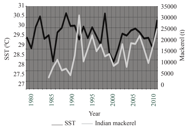
Fig. 4. Catch of Indian mackerel vs. SST along Tamil Nadu coast (1985-2010)
