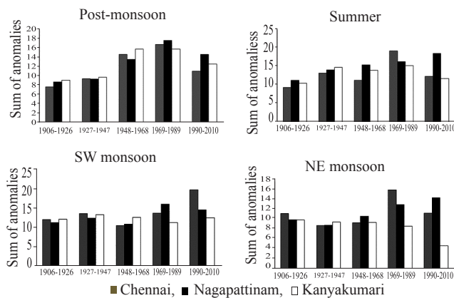
Fig. 2. Season-wise anomaly in SST in three regions of Tamil Nadu
