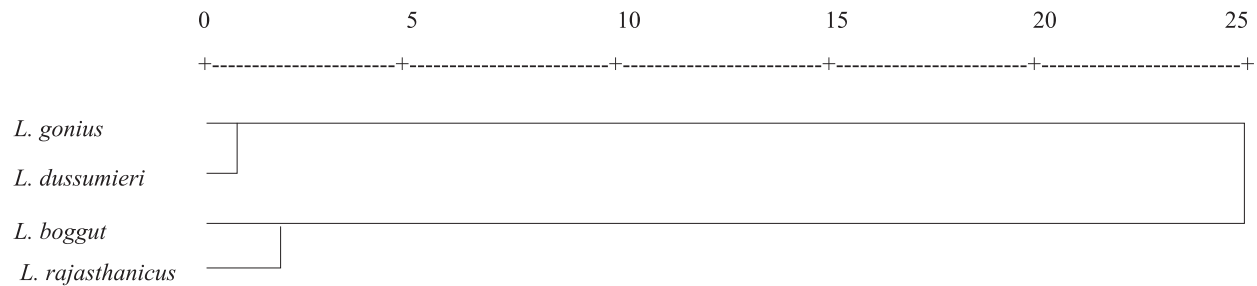
Fig. 7. UPGMA cluster analysis based on the Mahalanobis distance between the species centroids
