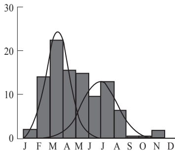
Fig. 6. Recruitment pattern of S. obtusata at Cochin
