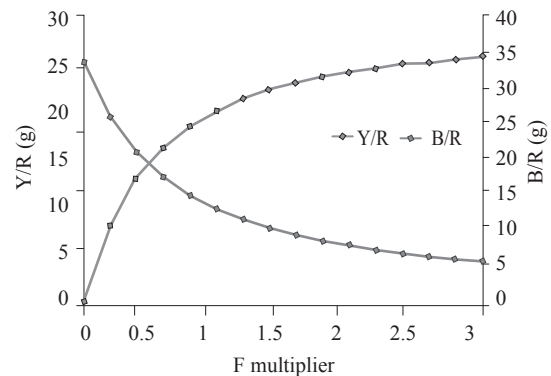
Fig. 8. Yield per recruit and biomass per recruit of S. obtusata for different multiples of F
