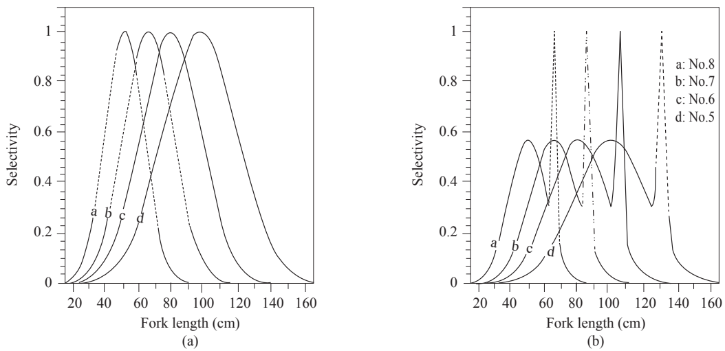
Fig. 2. Selectivity curves of better and best fit models for different hook sizes (a) Normal scale model (equal fishing power) - better fit Carangoides fulvoguttatus , (b) Bi-normal model (fishing power \alpha hook size) - best fit Carangoides fulvoguttatus
