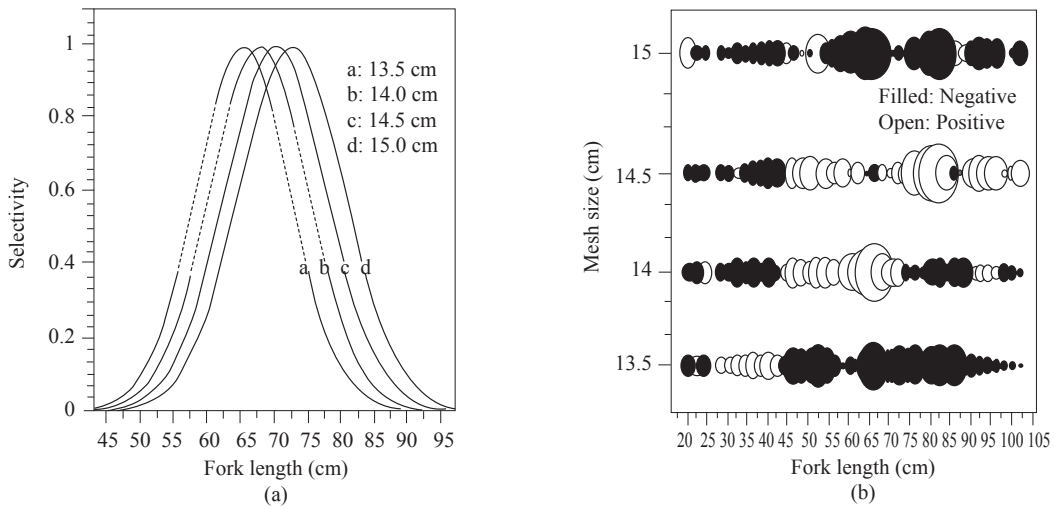
Fig. 1. Selective curve and residual plot of normal scale model (fishing power \alpha mesh size) of Carangoides fulvoguttatus (area of the circle is proportional to square of the residual)
