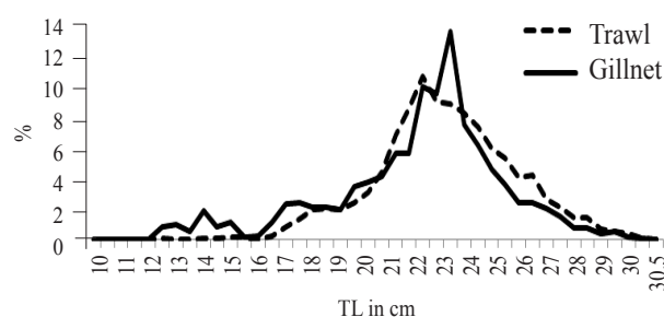
Fig. 2. Average annual length composition of R. kanagurta in Tuticorin during 2011-14
