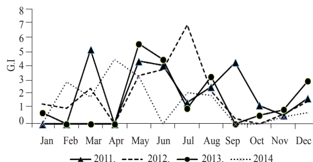
Fig. 5. Gonado-somatic index of R. kanagurta (sexes pooled)
