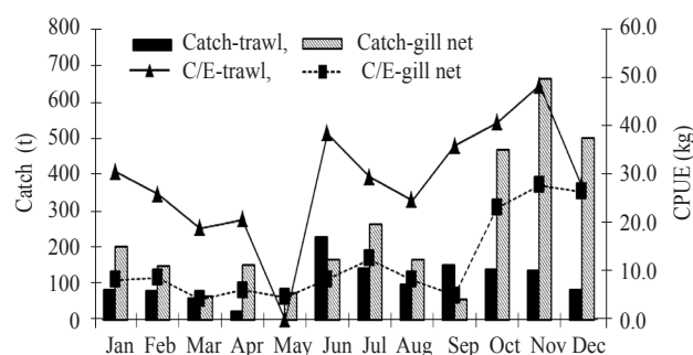
Fig. 1. Average gear-wise seasonal landing of R. kanagurta in Tuticorin during 2011-14
