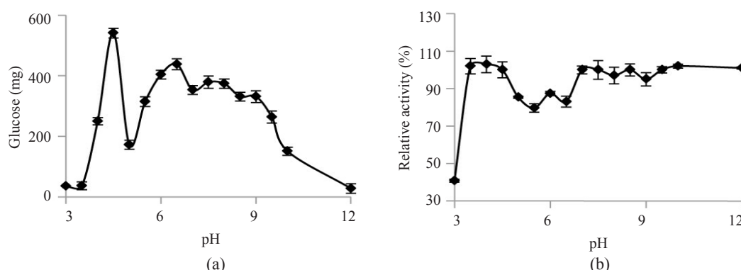
Fig. 4. Effect of (a) incubation pH and (b) pH stability on \alpha -amylase activity
