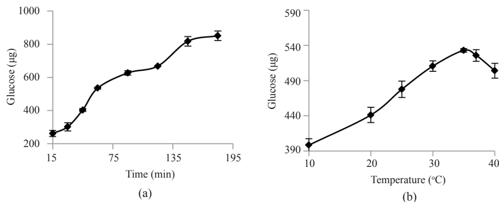
Fig. 2. Effect of (a) incubation time and (b) temperature on \alpha -amylase activity
