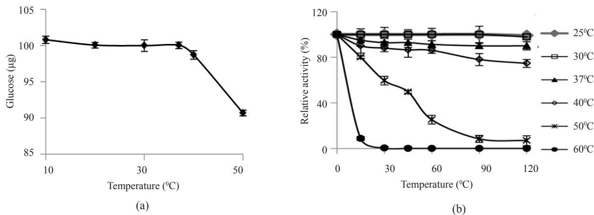
Fig. 3. Effect of (a) heat treatment and (b) thermostability on \alpha -amylase activity
