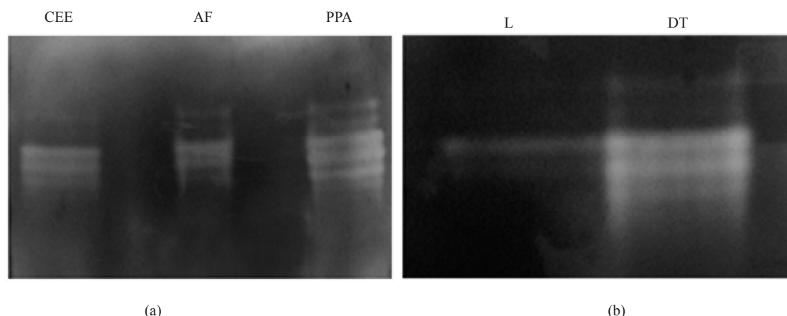
Fig. 6. Native PAGE gel showing amylase activities in substrate-stained (a) crude enzyme extract (CEE), acetone fraction (AF) and partially purified amylase (PPA); (b) Digestive tract (DT) and Liver (L).
