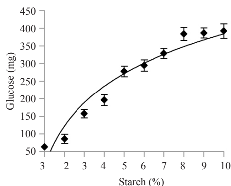
Fig. 5. Effect of starch concentration on \alpha -amylase activity
