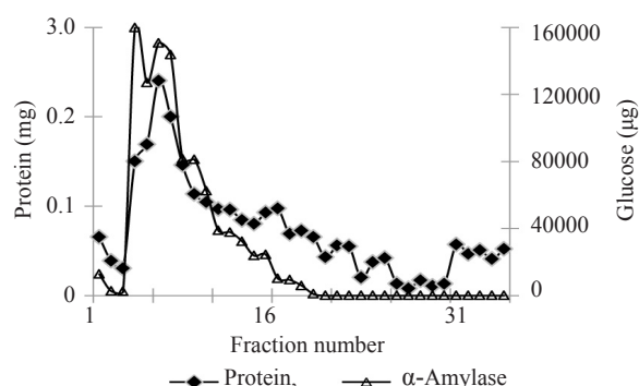
Fig. 1. Purification of \alpha -amylases by ion exchange chromatography
