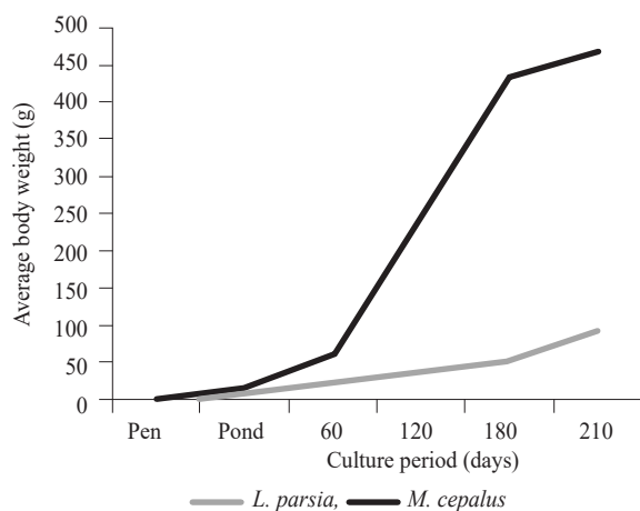
Fig. 1. Growth curve of two sympatric mullet species under same grow-out conditions
