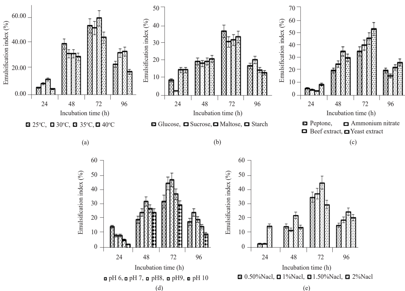
Fig. 4. Emulsification index* for biosurfactant production by Pseudomonas aeruginosa BHI 9 at different (a) temperatures; (b) carbon source; (c) nitrogen source; (d) pH and (e) NaCl. Incubation was carried out at 30°C at 125 rpm for 24, 48, 72 and 96 h. *Mean ± S.E, n=3
