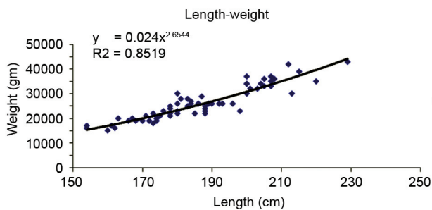
Fig. 1. Length (LjFL)-weight relationship of I. platypterus from south-eastern Arabian Sea
