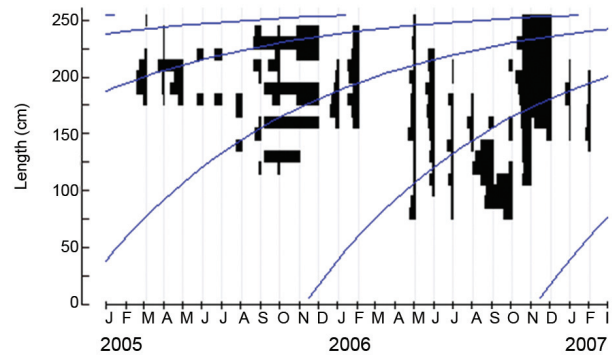
Fig. 2. Growth parameters L_\infty = 261 cm and annual K=1 of I. platypterus estimated in ELEFAN
