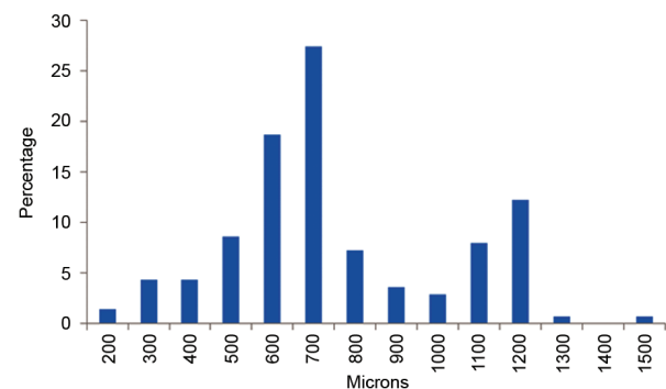
Fig. 3. Oocyte size distribution of a ripe ovary of I. platypterus
