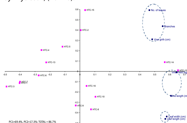
Fig. 6: Association analysis among morphological traits (2 nd year).
