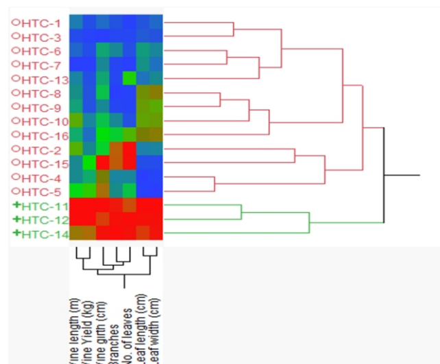
Fig. 7: Two way multivariate hierarchical clustering of genotypes vis-à-vis measures by Ward's method (1 st year).
