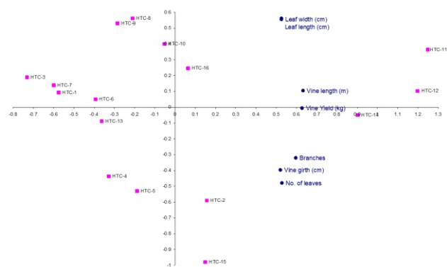
Fig. 4: Association analysis among morphological traits (1 st year).
