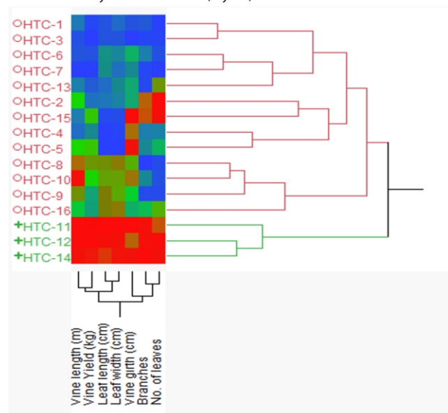
Fig. 8: Two-way multivariate hierarchical clustering of genotypes vis-à-vis morphological traits by Ward's method (2 nd year).
