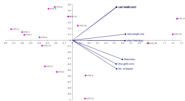
Fig. 3: Biplot analysis of morphological traits and genotypes (1 st year).
