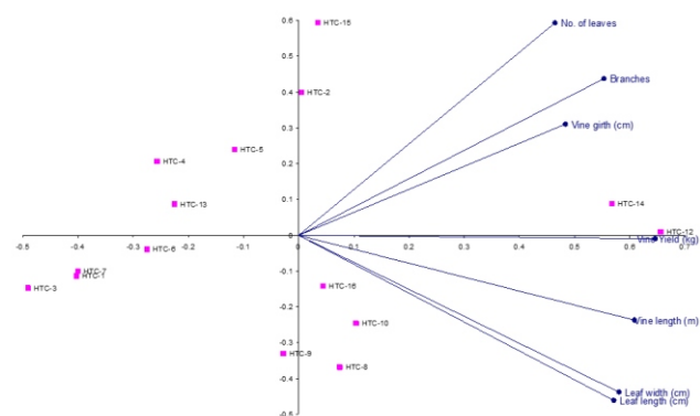
Fig. 5: Biplot analysis of morphological traits and evaluated genotypes (2 nd year).
