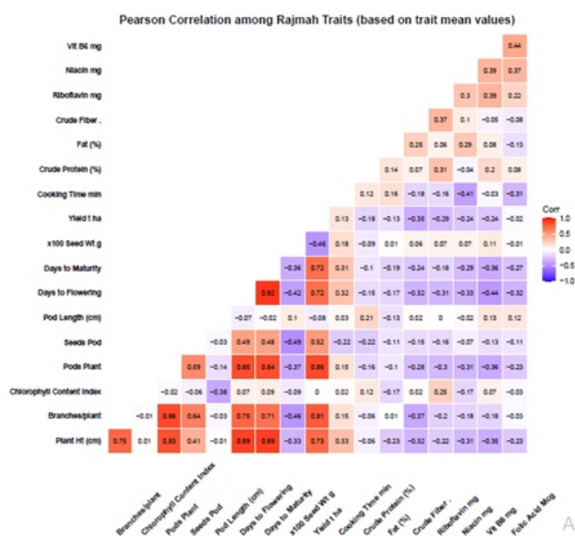
Fig. 1: Pearson correlation heatmap showing associations among 18 morphological and biochemical traits in 40 rajmah genotypes.
