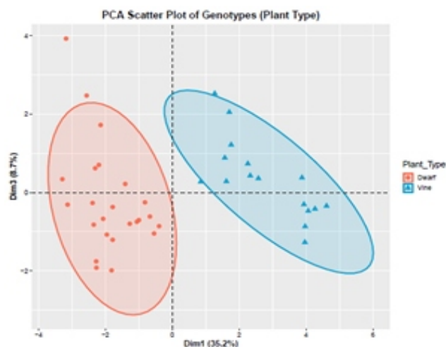
Fig. 4: PCA scatter plot of genotypes based on 18 traits (PC1 vs PC3), color-coded by plant type (Dwarf and Vine).
