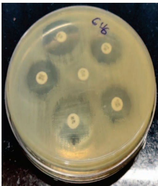
Fig. 4. Antibiotics sensitivity testing of E. coli on Mueller Hinton Agar.
