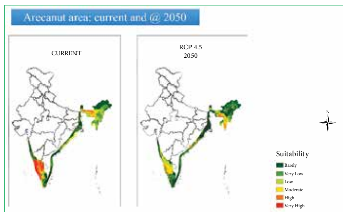
Prediction of arecanut area in future climate by Biomod2 model
