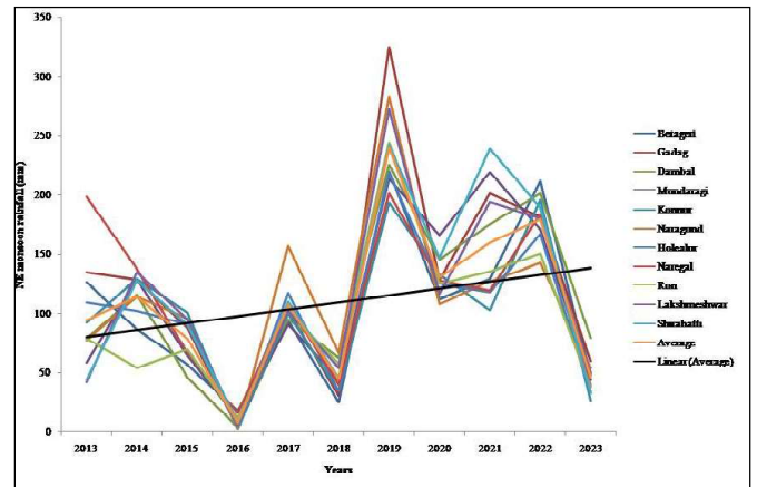
Fig 8. NE monsoon (October to December) rainfall at Hoblis across Gadag district (2013-2023)
