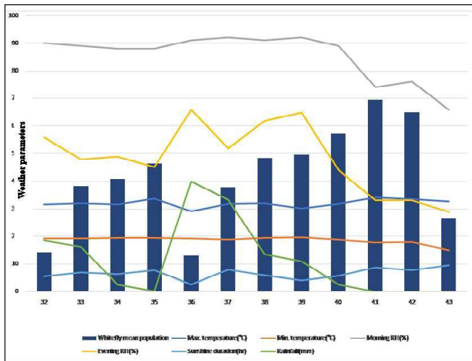
Fig. 1. Relation between weather parameters and mean population of whitefly ( Bemisia tabaci ) transmitting YMD of blackgram at different SMWs
