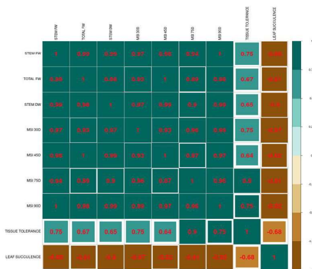
Fig 2. Heat map of Pearson's correlation coefficients of morphological and physiological parameters calculated for four PMN hybrid genotypes under salinity. n=4; at 5% P=0.95. FW=fresh weight, DW= dry weight, MSI = Membrane stability index
