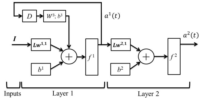
Fig. 1. A two-layered LRNN architecture
