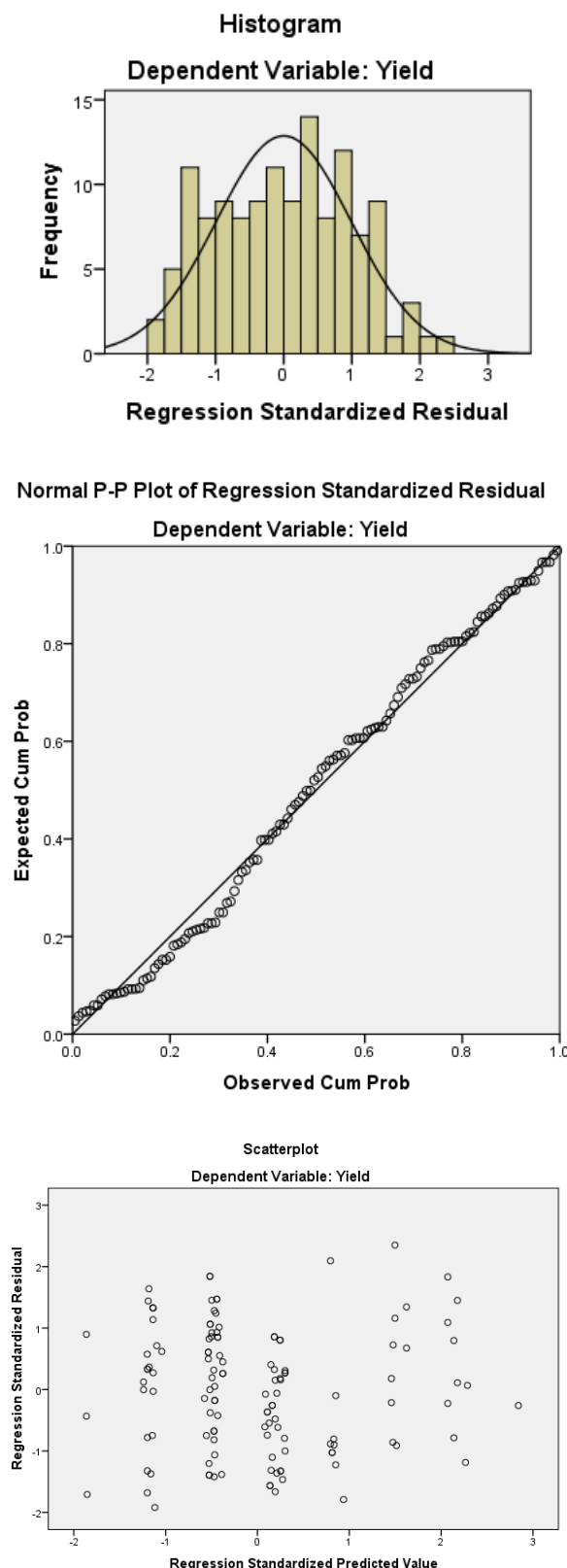
Fig. 5. Regression diagnostics of the selected zonal yield forecast model. (CCT+ weather variables)
