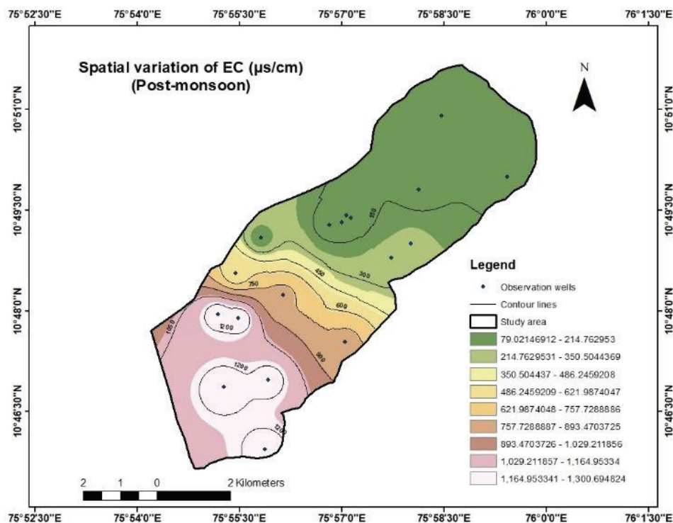
Fig. 11. Spatial variation of EC (Post-monsoon)
