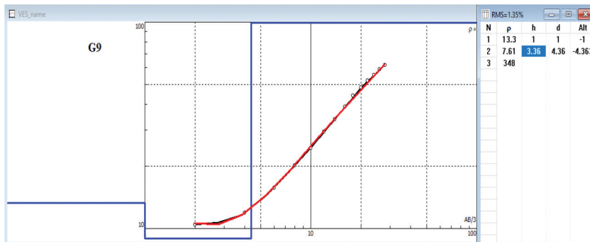
Fig. 7a. Sounding curve of the location G9 (H-Type)
