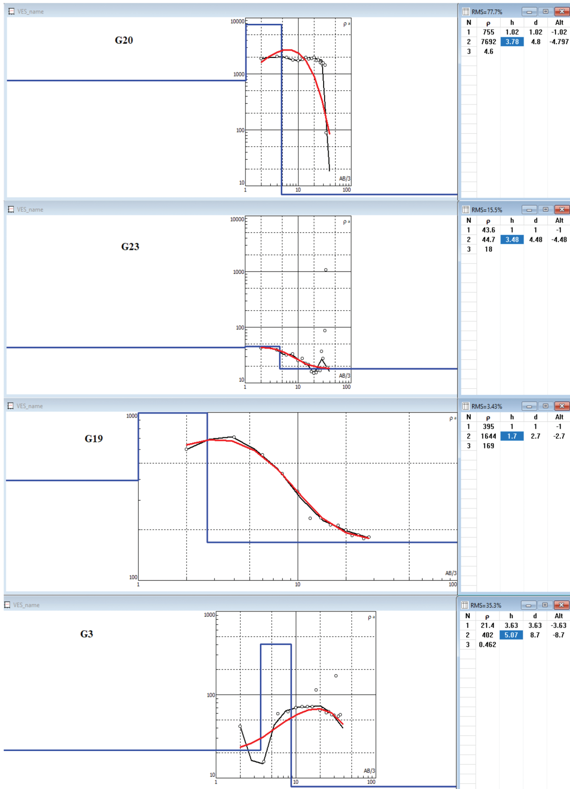
Fig. 8. Sounding curves of the location G19, G3, G20 and G23 (K-Type)
