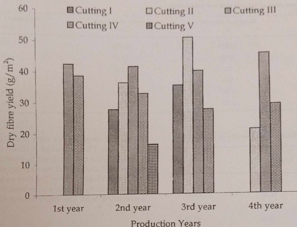
Fig. 1 Cutting and production year wise dry fibre yield (g m 2 )
