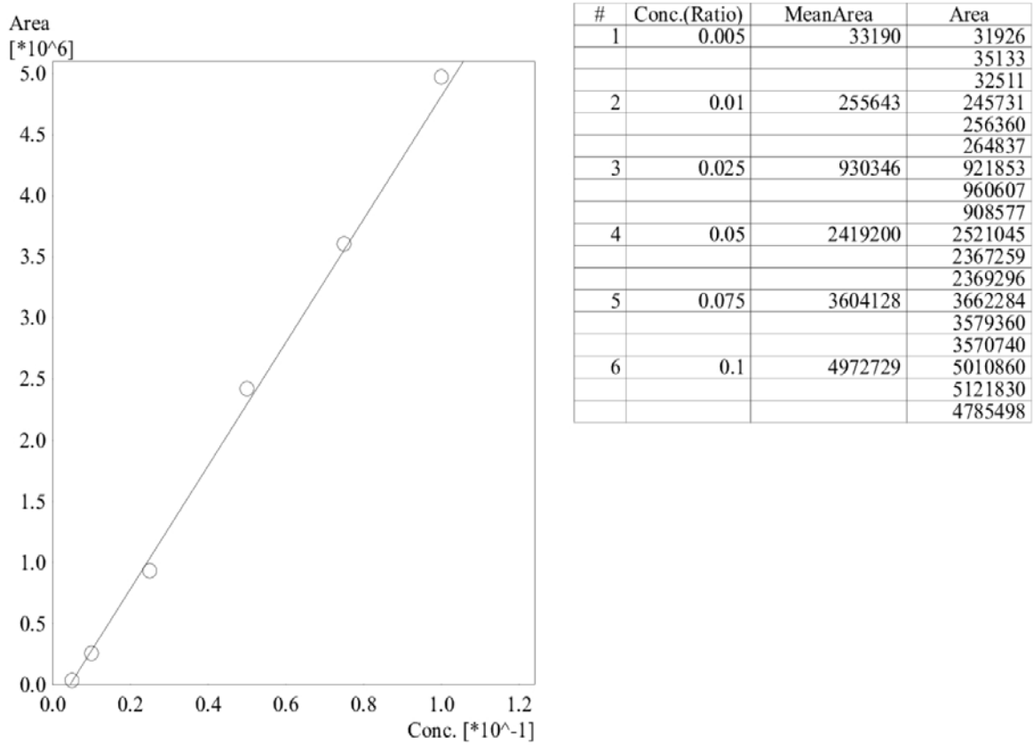
Fig. 5. Linearity curve of emamectin benzoate (0.005-0.1ppm)
