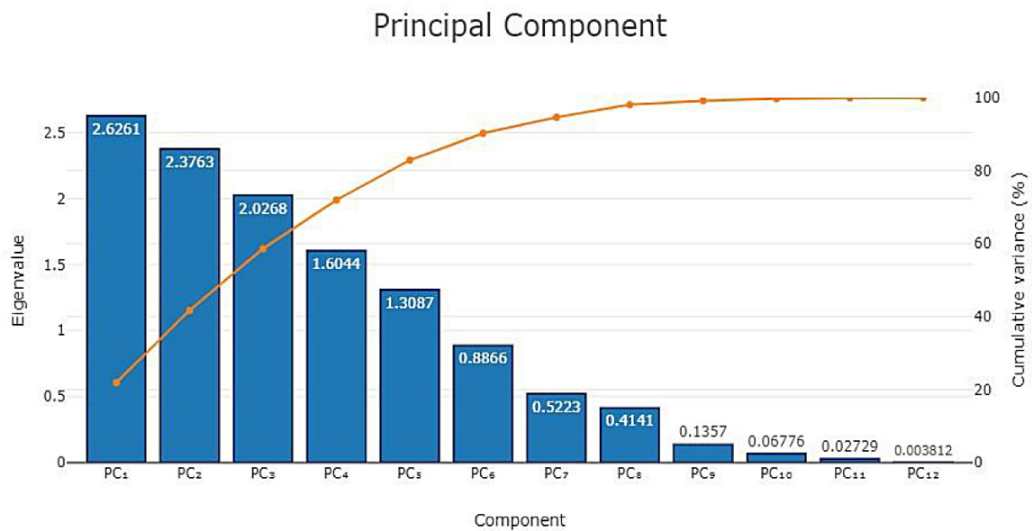
Figure 6. Scree plot Curve Depicting the variation in PC Score among the BTM lines
